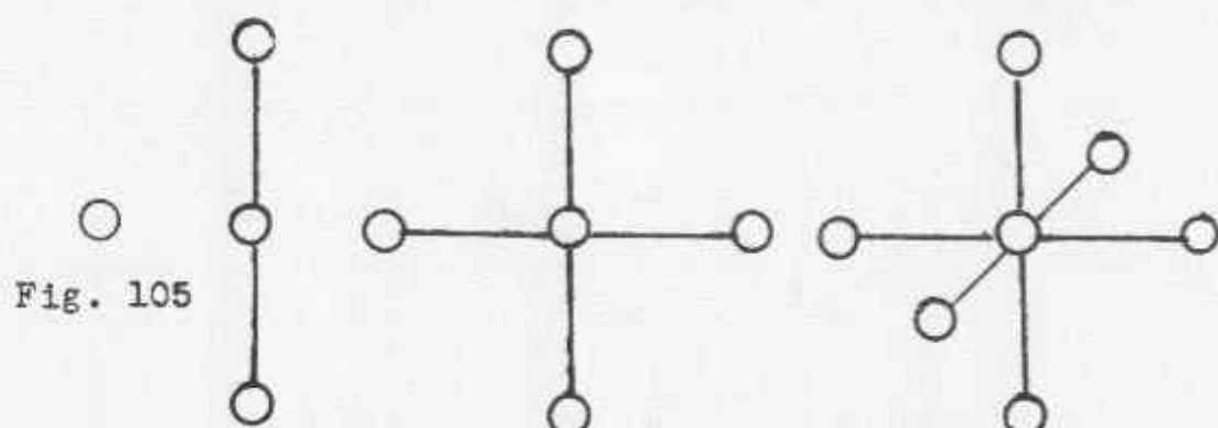
Fig. 106. Fig. 107. Fig. 108. THE NINE ZEROS WHICH BOUND THE THREE PROJECTION MIRRORS WHICH CAUSE THE ILLUSION OF A THREE DIMENSIONAL UNIVERSE.
