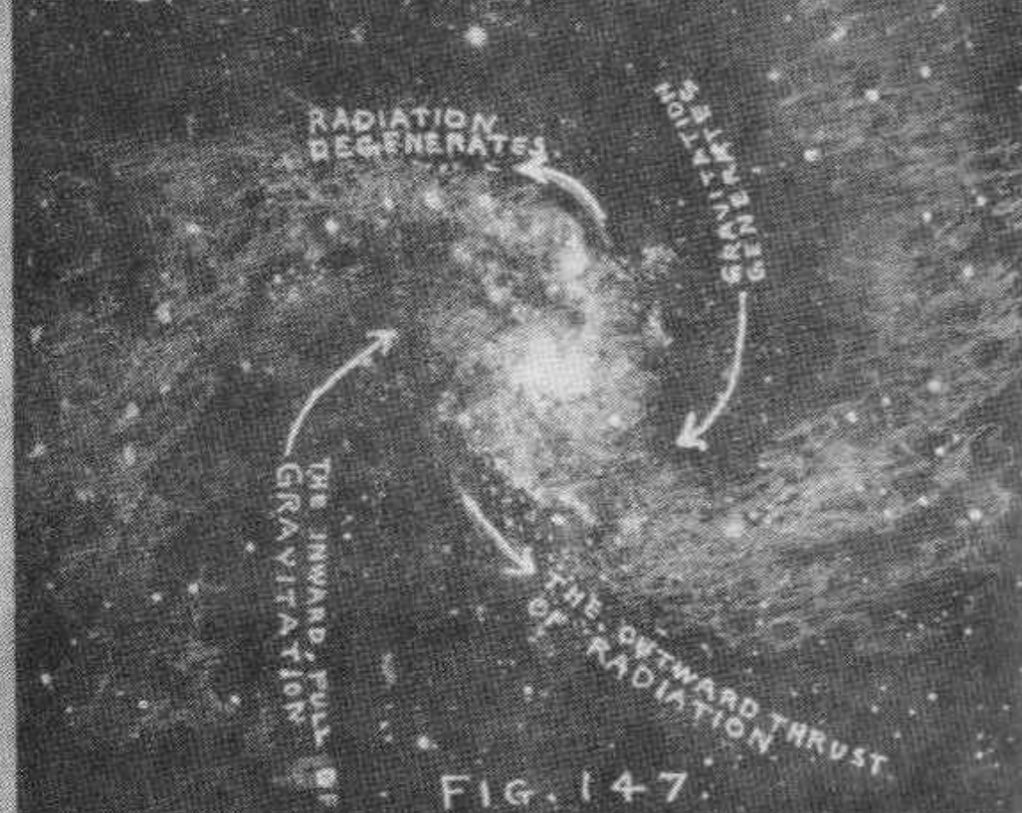
SPIRAL NEBULA M. 33, TRIAGULI,
