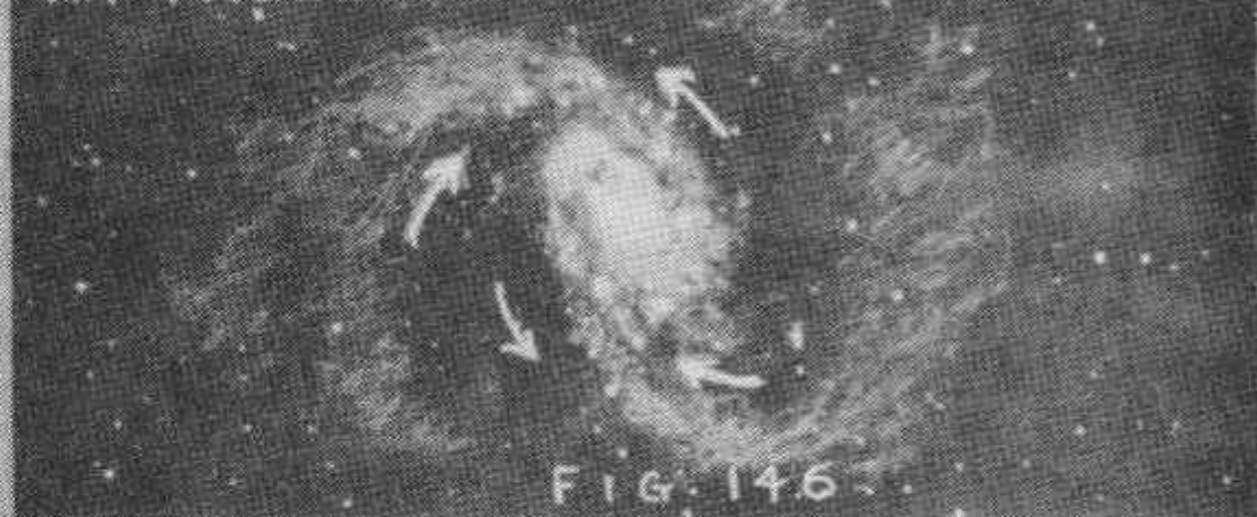
SPIRAL NEBULA M.V. 44, CAMELOPARD
